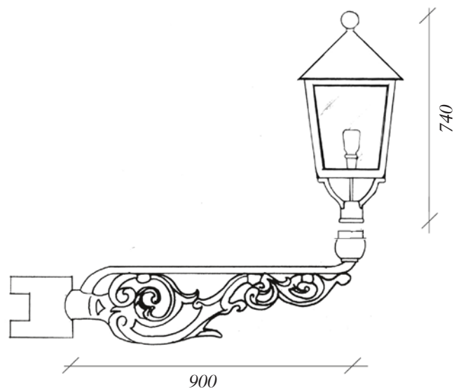
Lykthus modell D
